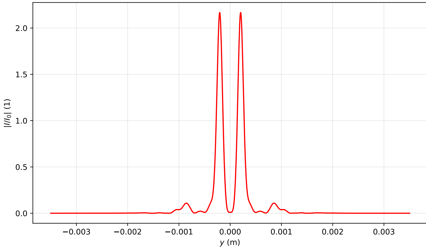
Intensity profile I(x=0, y, z=1.194)/I_0 , P_{in}=5.5P_{cr} , artificial time
